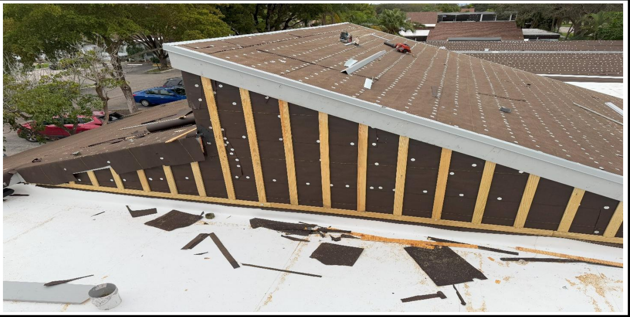
8 – Ongoing, Installation of the fascia board / drip edges / siding wood strips, BLDG 07.
