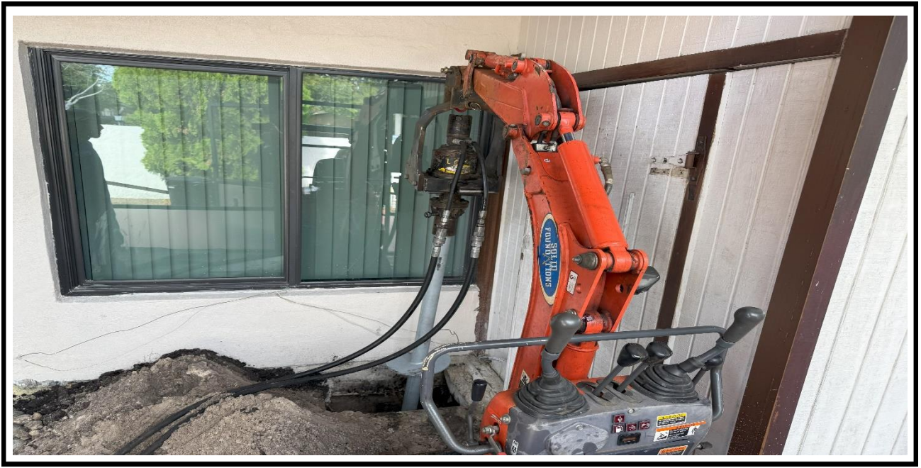
15 – Ongoing, Ongoing, Installation of the helical piles, BLDG 20.
