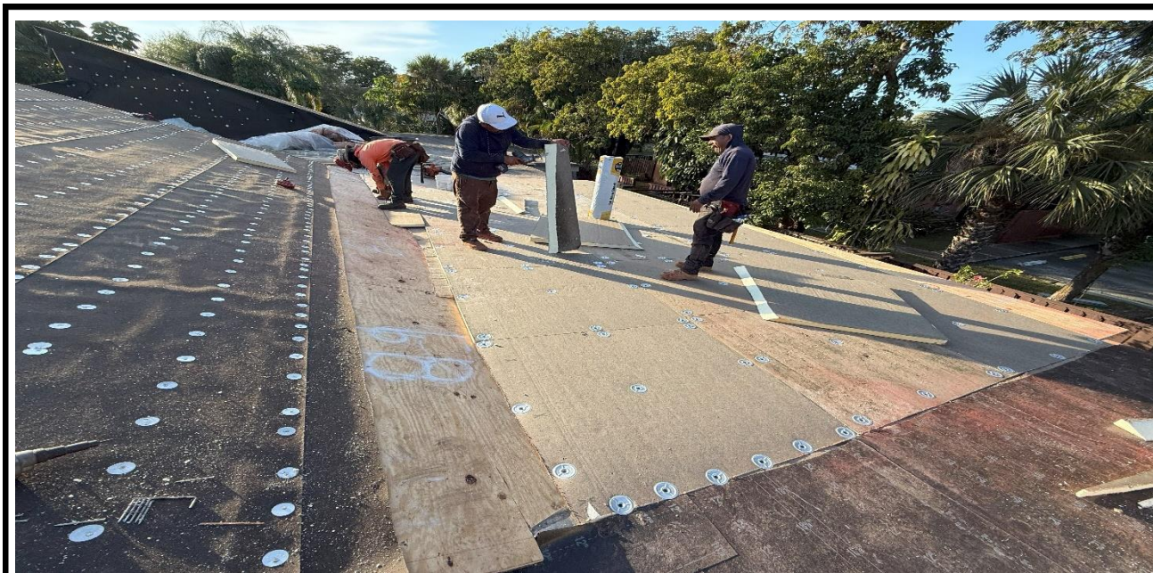
1 – Ongoing, Laying down the insulation sheets on top of the plywood and adding the tin caps, BLDG 02.
