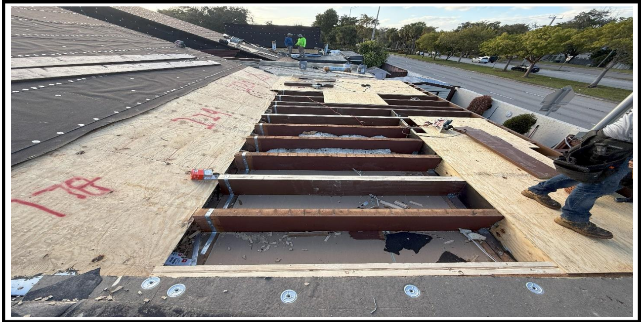
8 – Ongoing, Installation of the new plywood and wood beams, BLDG 15.
