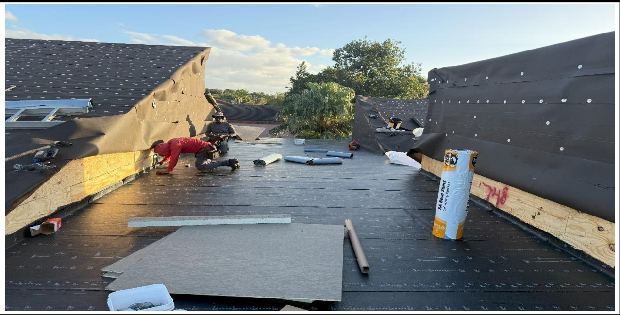
12 – Ongoing, Laying down the waterproof black paper on top of the plywood and adding the tin caps, BLDG 15.
