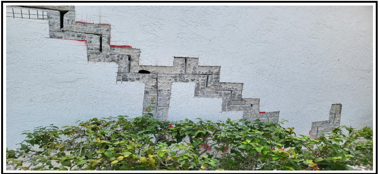
1 – Cutting and chipping of the delaminated and cracked stucco at the exterior walls.
