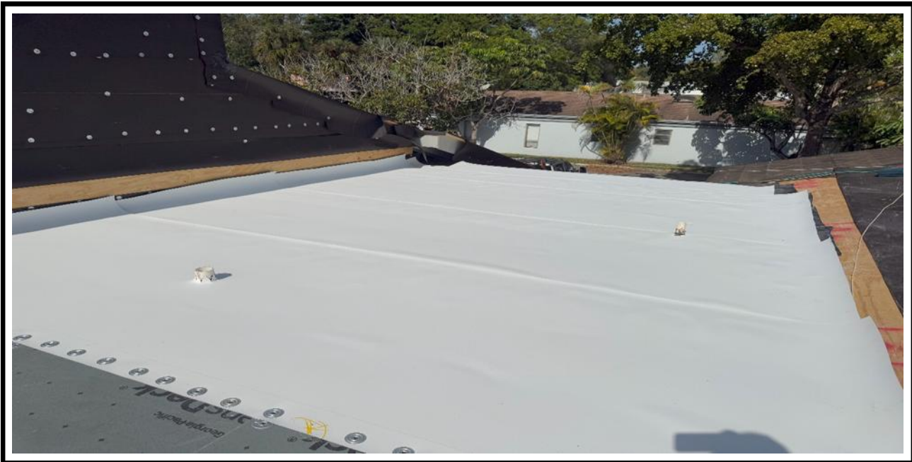
11 – Ongoing, laying down the TPO sheets and welding it, BLDG 09.
